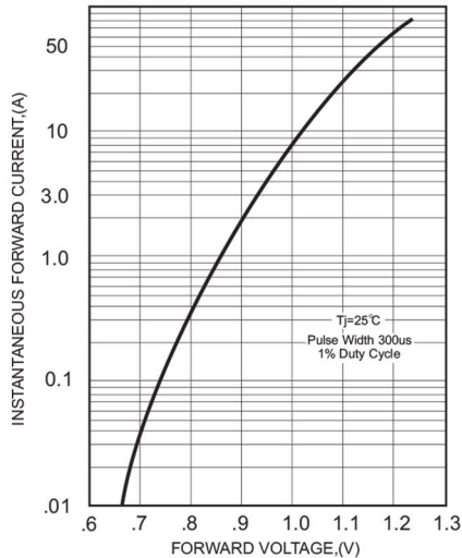
FIG.1-TYPICAL FORWARD CHARACTERISTICS
